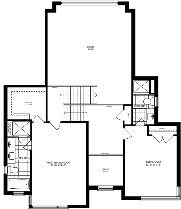
Second Floor ELEVATION 'B'
